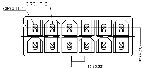
2~22 Circuits
