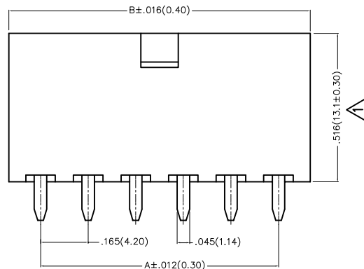
2~22 Circuits
