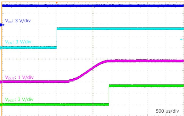
Figure 56. EN Start-up at No Load (VIN = 5.0 V, VOUT = 1.8 V, VEN = 0 V to 5 V)
