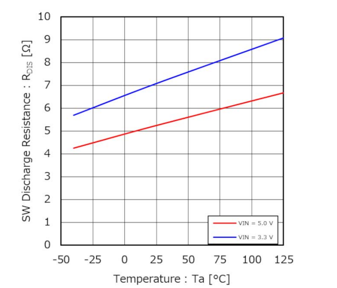
Figure 14. SW Discharge Resistance vs Temperature
