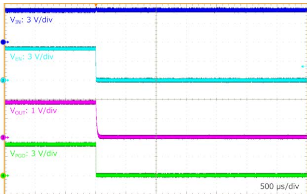
Figure 59. EN Shutdown at RLoad = 0.6 Ω (VIN = 5.0 V, VOUT = 1.8 V, VEN = 5 V to 0 V)
