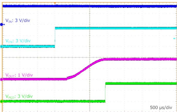
Figure 58. EN Start-up at RLoad = 0.6 Ω (VIN = 5.0 V, VOUT = 1.8 V, VEN = 0 V to 5 V)
