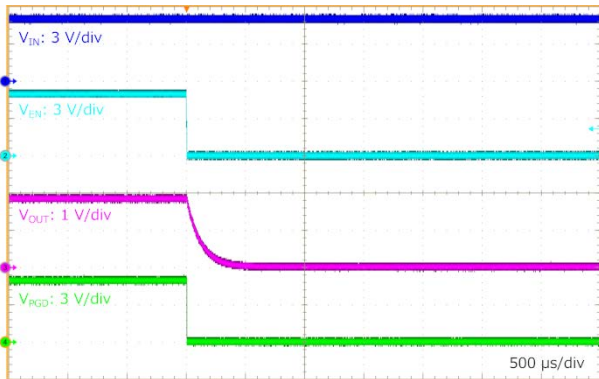
Figure 57. EN Shutdown at No Load (VIN = 5.0 V, VOUT = 1.8 V, VEN = 5 V to 0 V)
