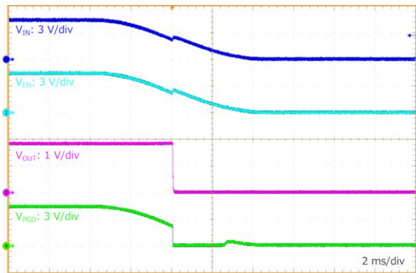
Figure 63. VIN Shutdown at R_{Load} = 0.6 \Omega ( V_{IN} = V_{EN} = 5 V to 0 V, V_{OUT} = 1.8 V)
