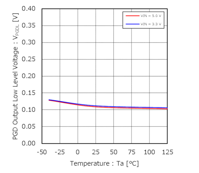
Figure 16. PGD Output Low Level Voltage vs Temperature
