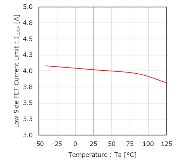
Figure 13. Low Side FET Current Limit vs Temperature
