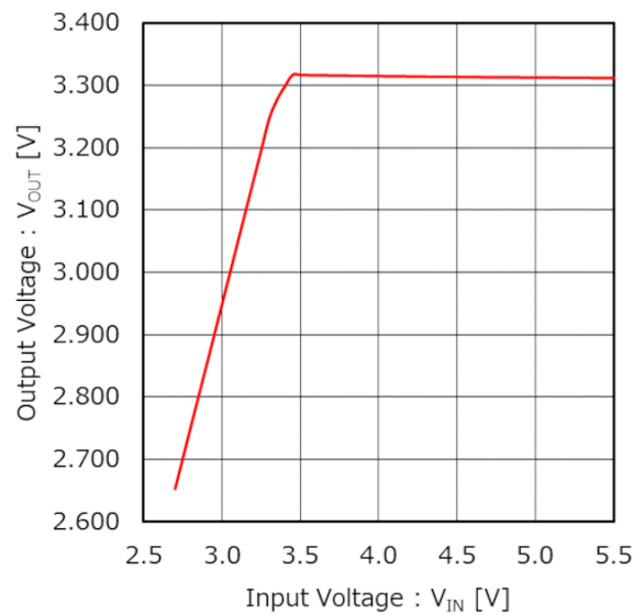
Figure 44. Output Voltage vs Input Voltage (Line Regulation) ( V_{OUT} = 3.3\text{ V} , I_{OUT} = 1.0\text{ A} )
