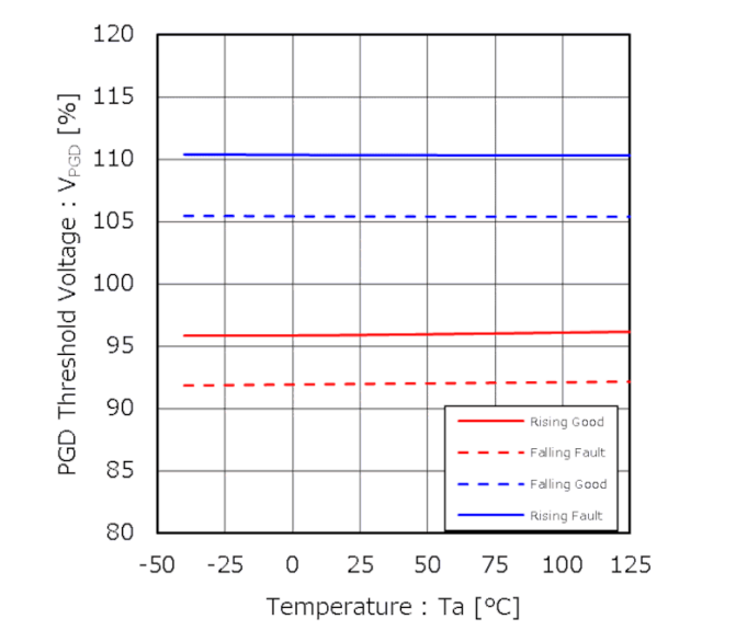
Figure 15. PGD Threshold Voltage vs Temperature
